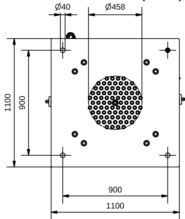
Bottom view (1:20)
